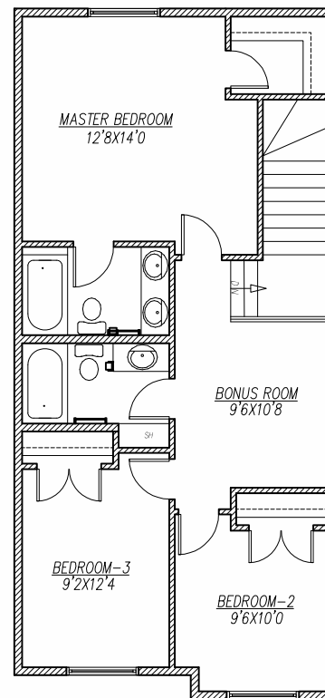
UPPER FLOOR PLAN 844 SQ.FT.
