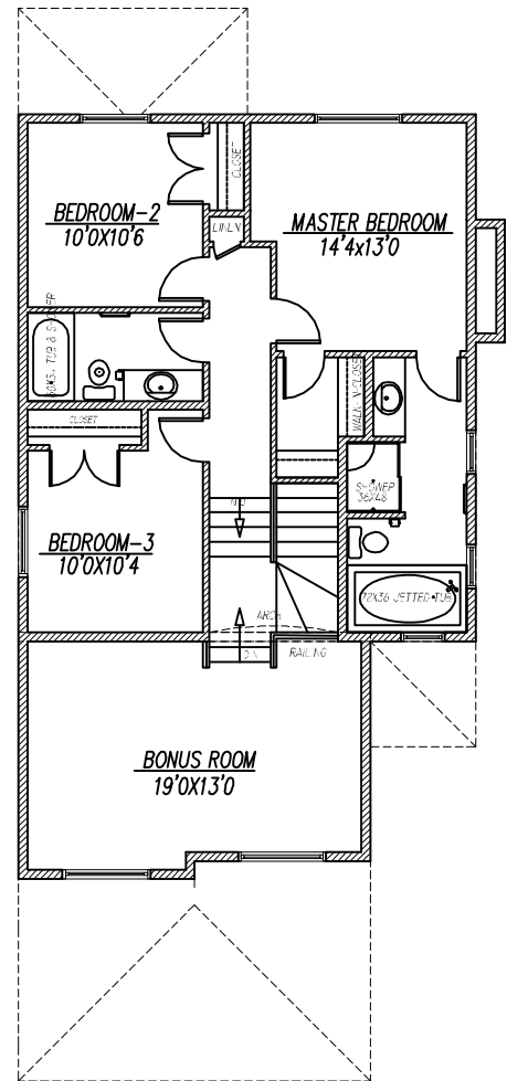
UPPER FLOOR PLAN 1040 SQ.FT.
