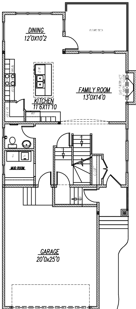
MAIN FLOOR PLAN 845 SQ.FT.
