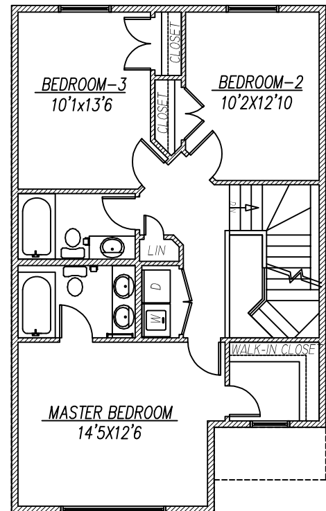
UPPER FLOOR PLAN 852 SQ.FT.
