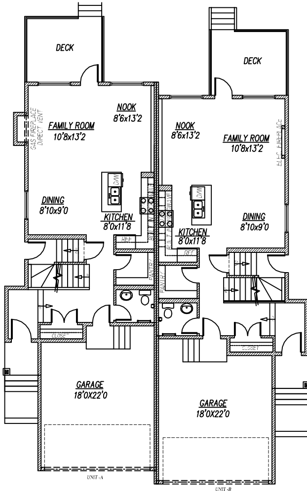
MAIN FLOOR PLAN 797 SQ.FT. (UNIT A)
