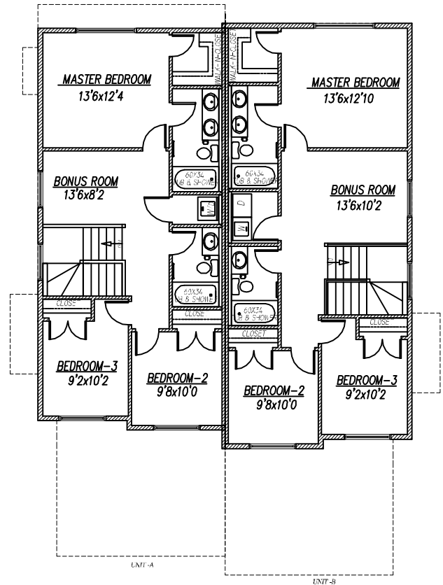
UPPER FLOOR PLAN 851 SQ.FT. (UNIT A)
